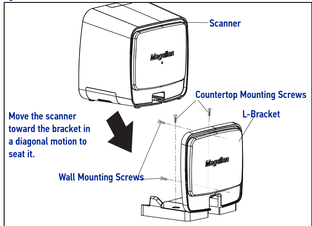
Figure 7. L-Bracket Mount
