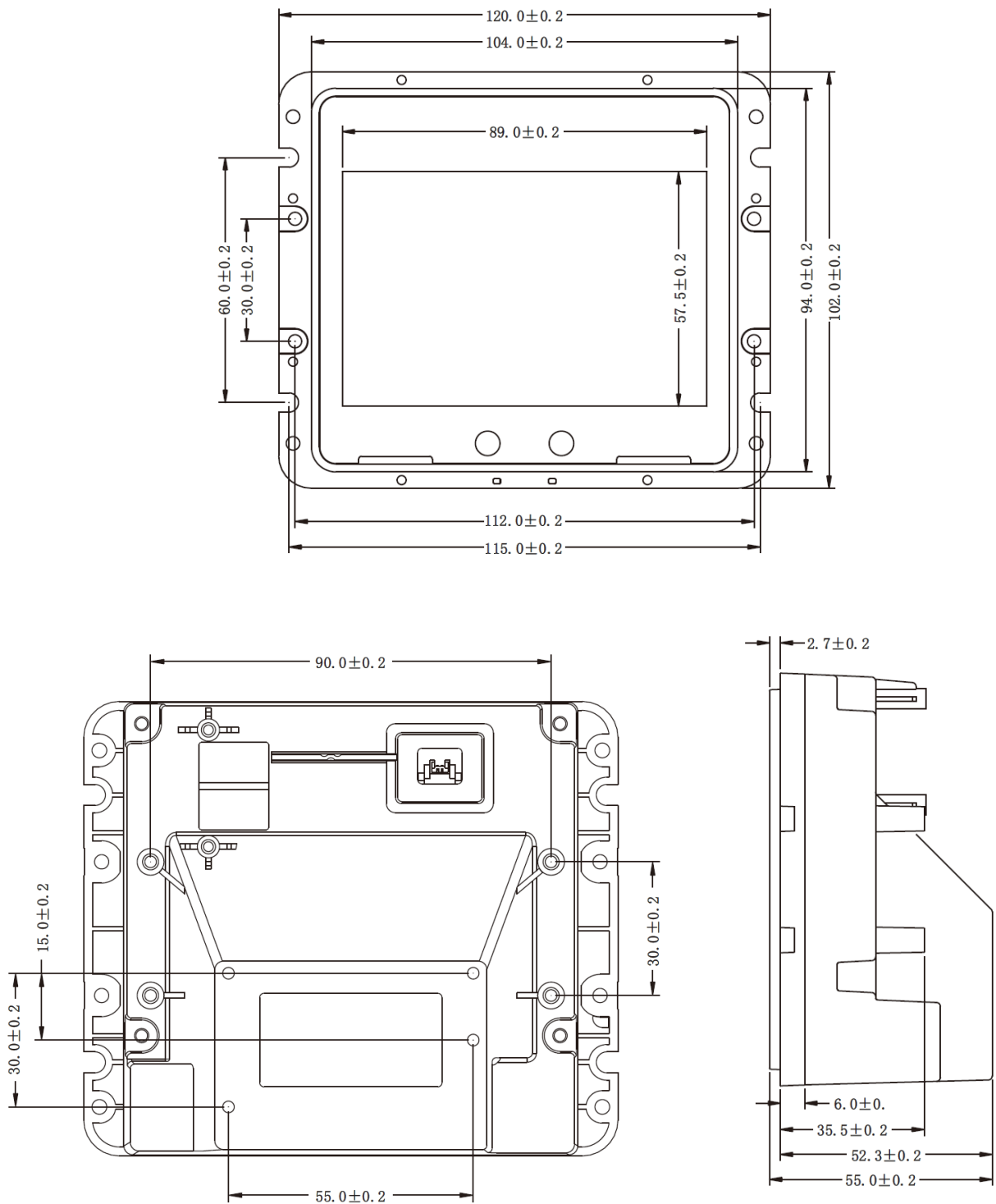
Figure 2-2 Dimensions
